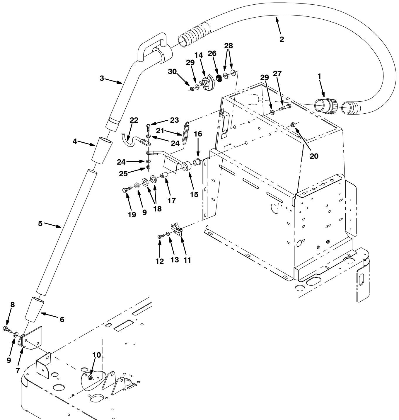
Fig. 2 – Vacuum Wand Group — Handsauger-Gruppe — Ensemble manche d'aspiration
