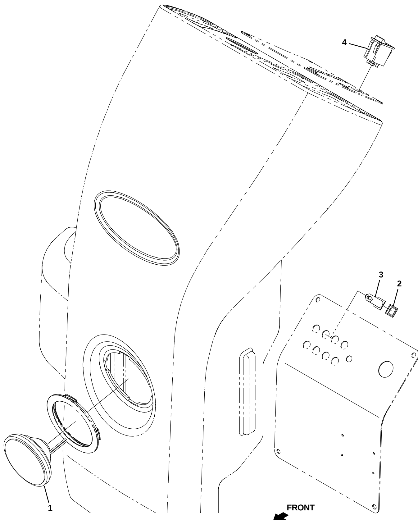
Fig. 1 – Headlight Kit
