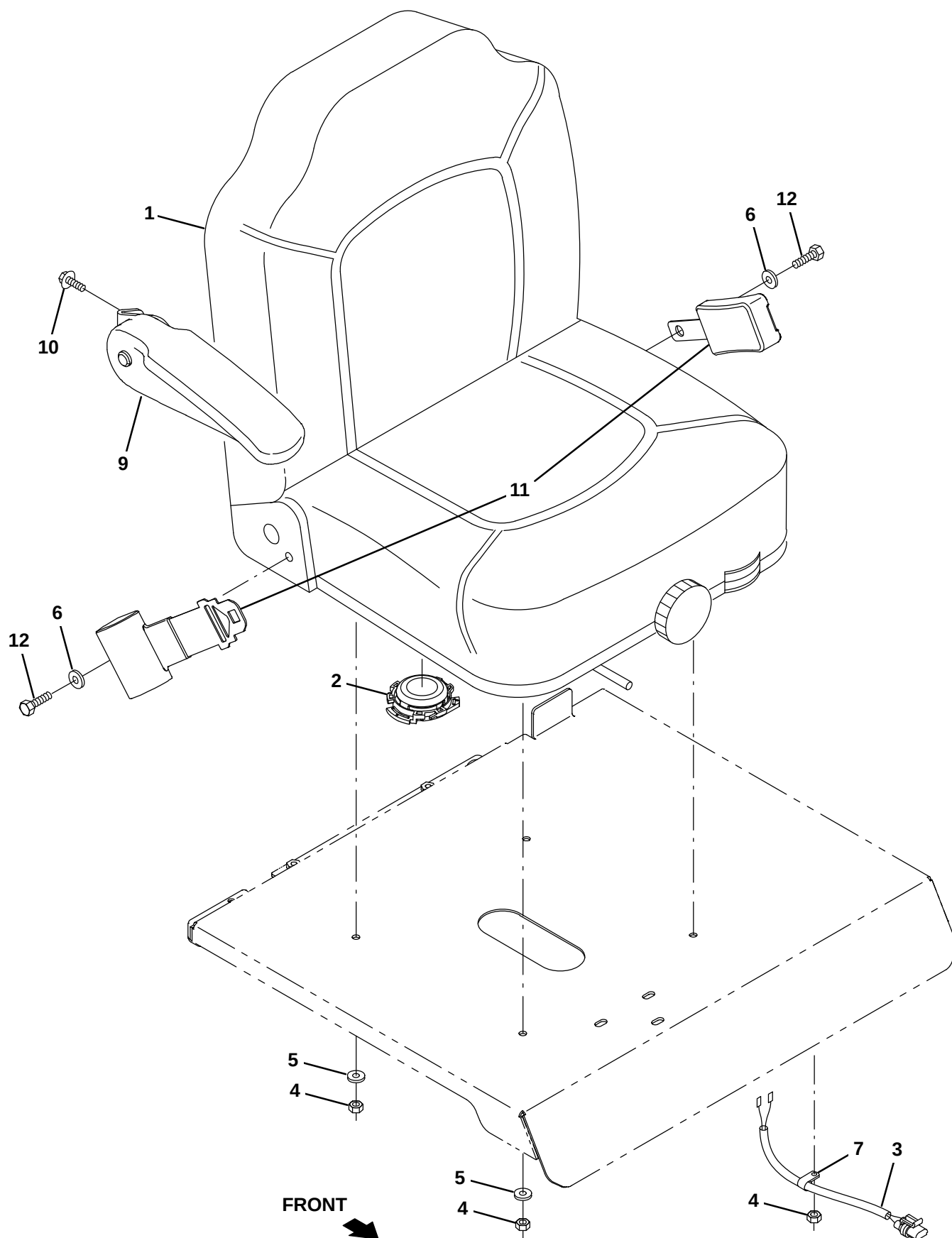
Fig. 24 – Deluxe Seat Group
