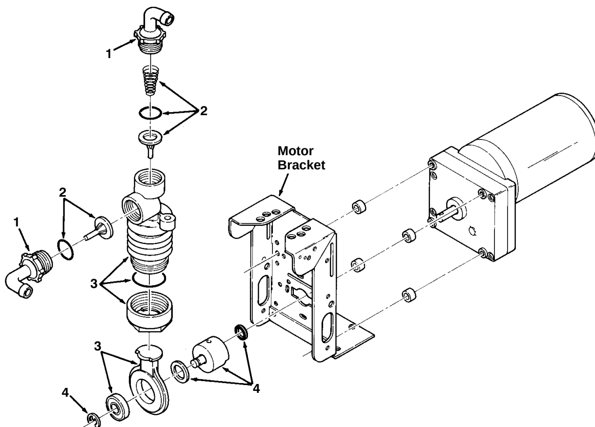
Fig. 10 – Metering Solution Pump Breakdown, 386364
