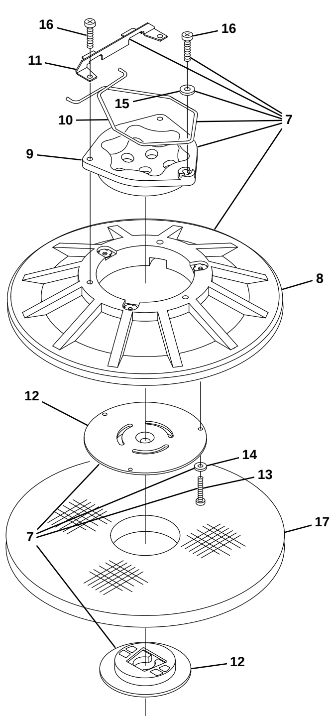
Fig. 1 – Replacement Brushes, Scrub Head
