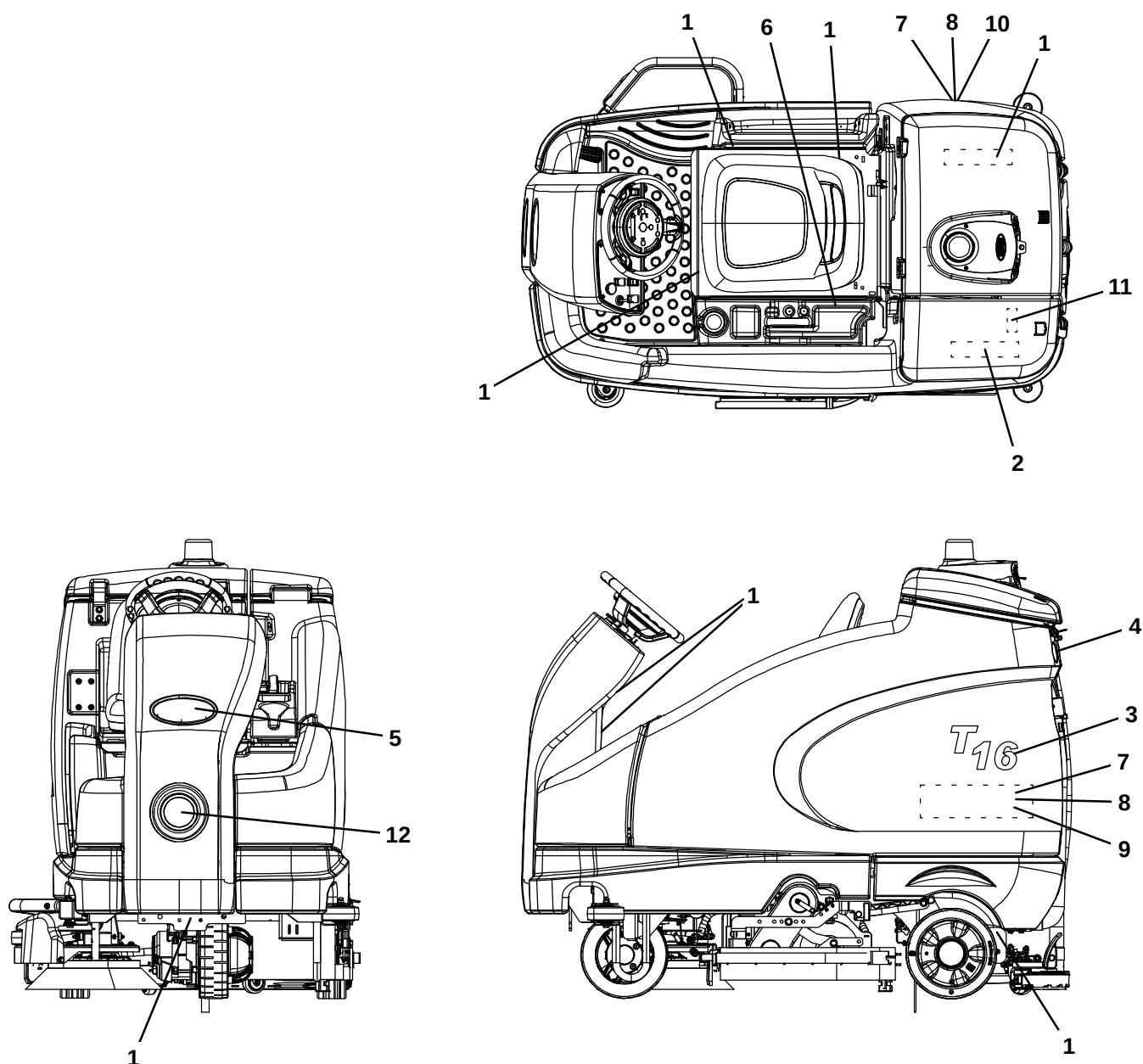
Fig. 24 – Label Group
