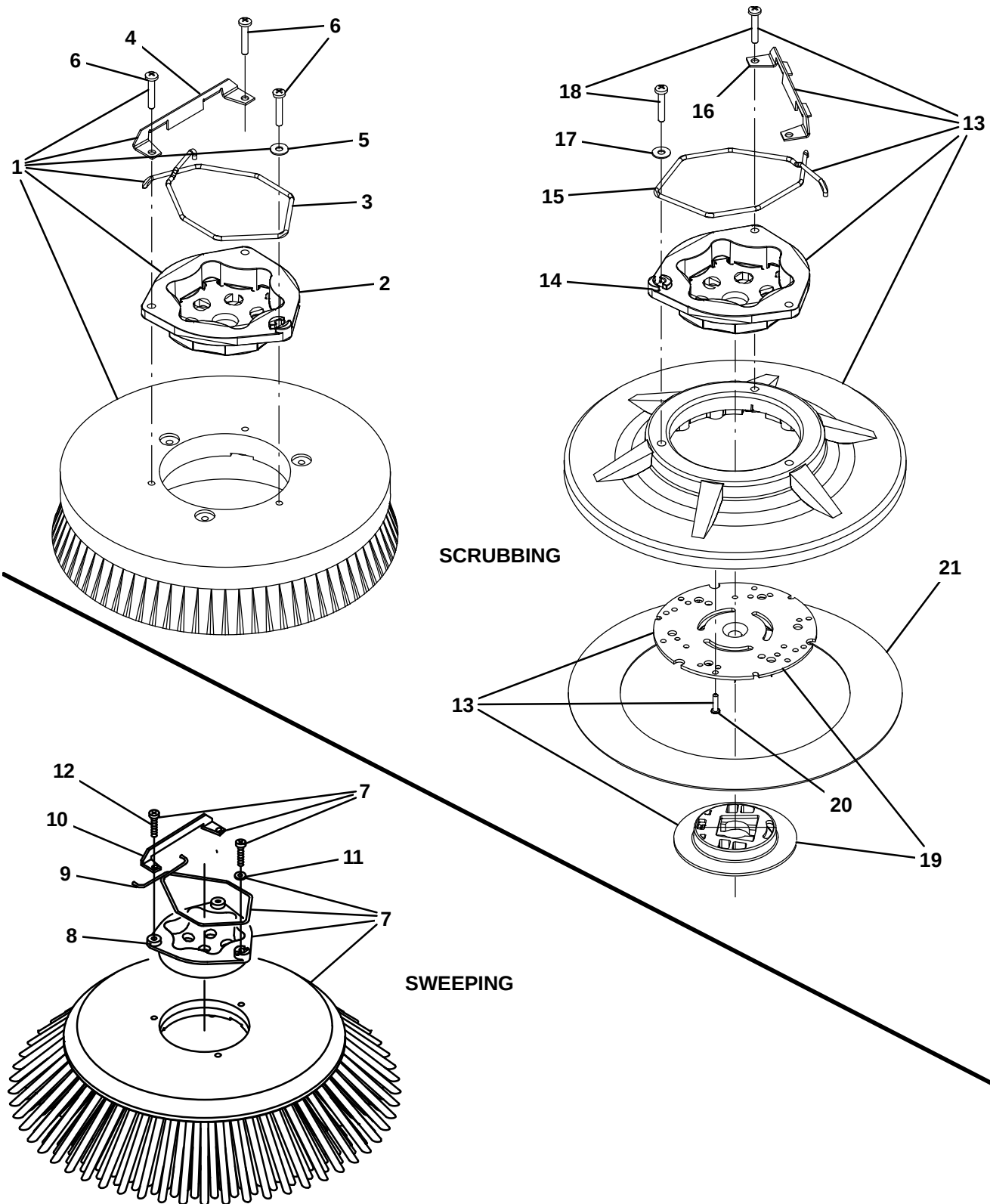
Fig. 2 – Replacement Brushes, Side Brush
