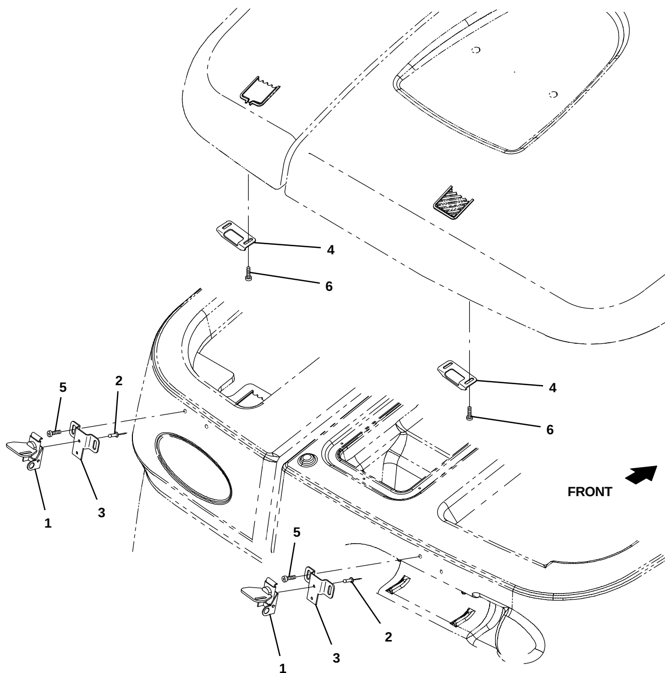
Fig. 25 – Transport Group
