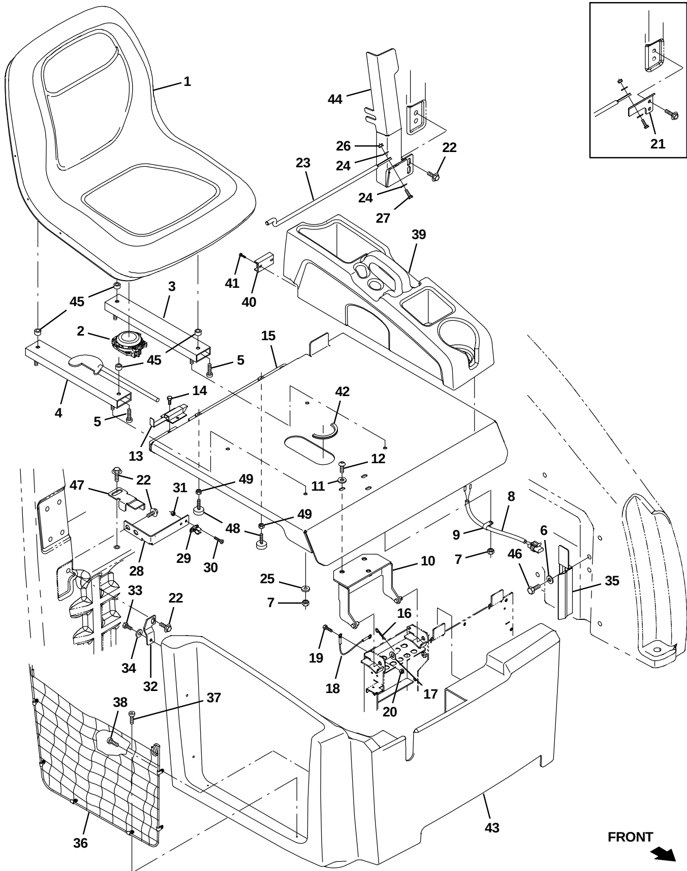
Fig. 4 – Seat Group
