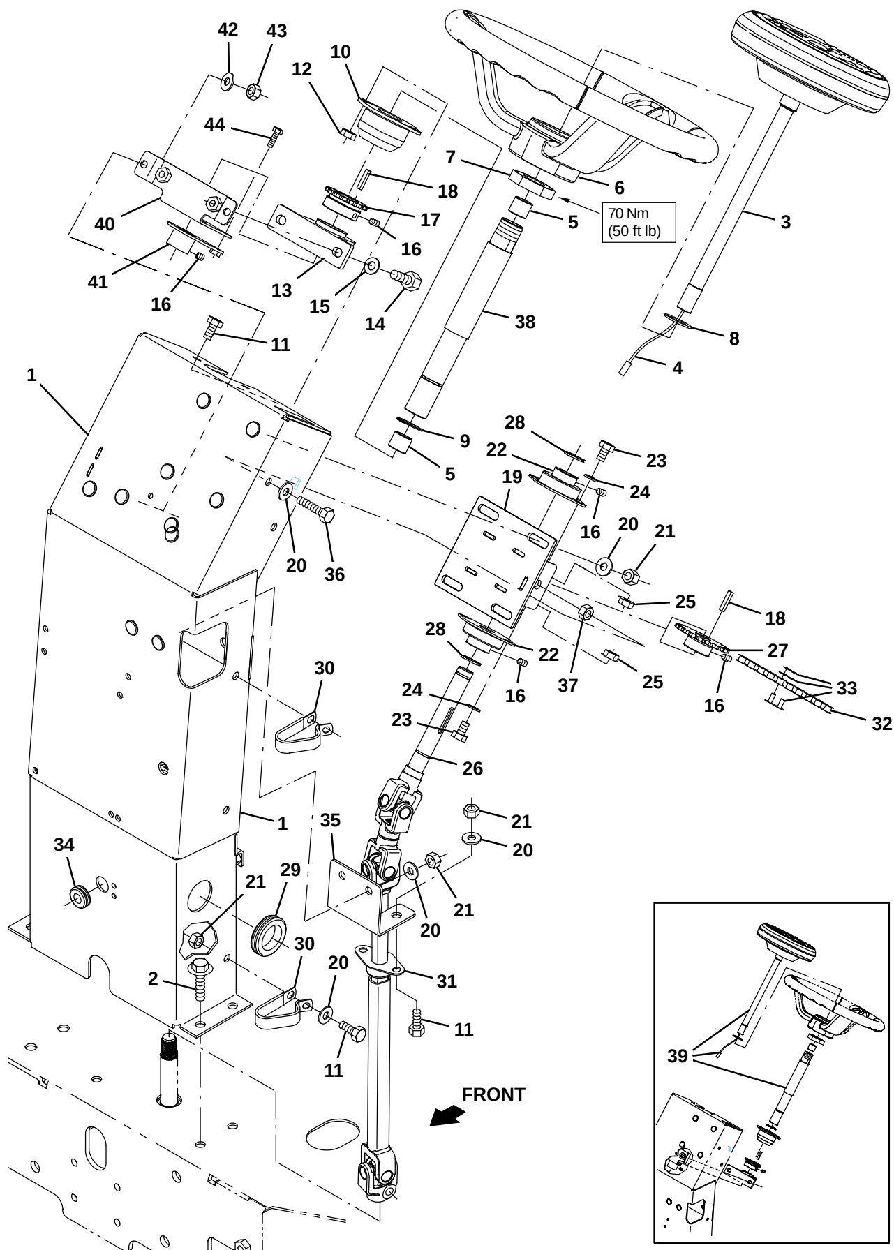
Fig. 5 – Steering Group
