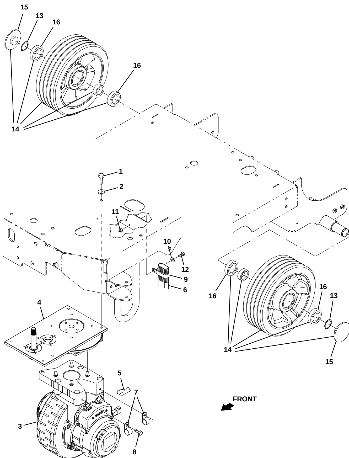
Fig. 9 – Wheels Group
