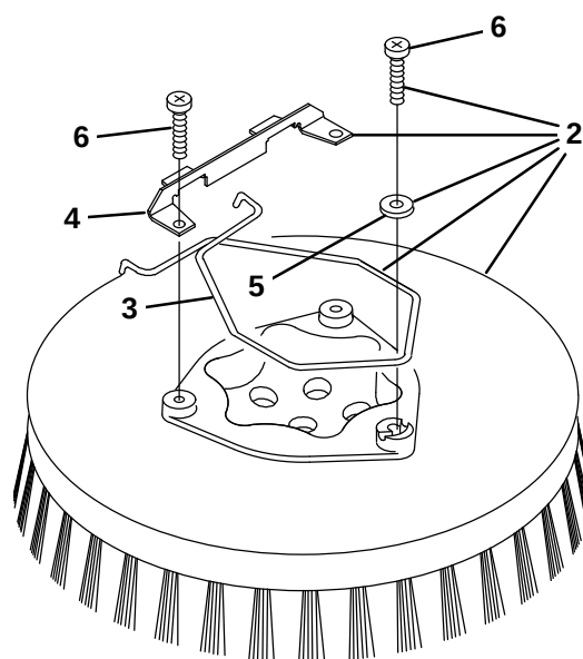
Fig. 1 – Replacement Brushes, Scrub Head
